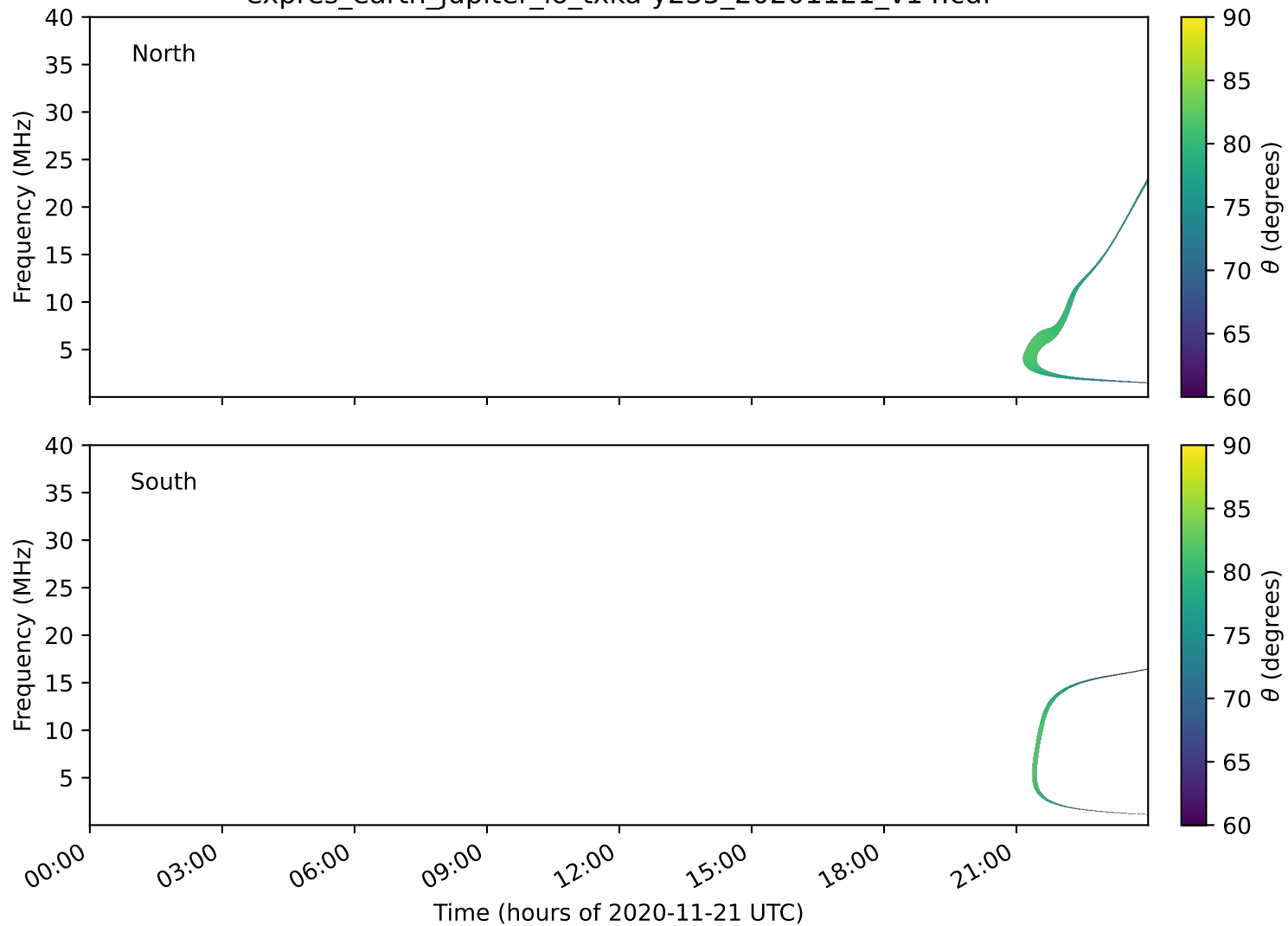
expres_earth_jupiter_io_txka-y235_20201121_v14.cdf
