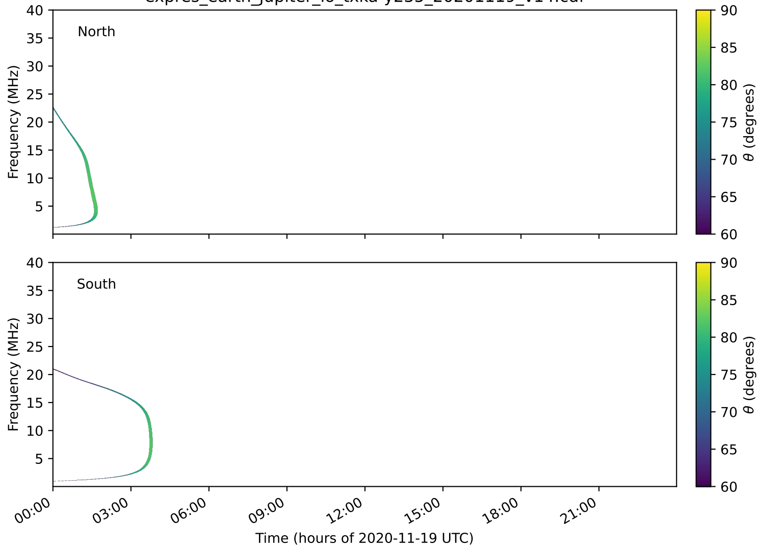
expres_earth_jupiter_io_txka-y235_20201119_v14.cdf
