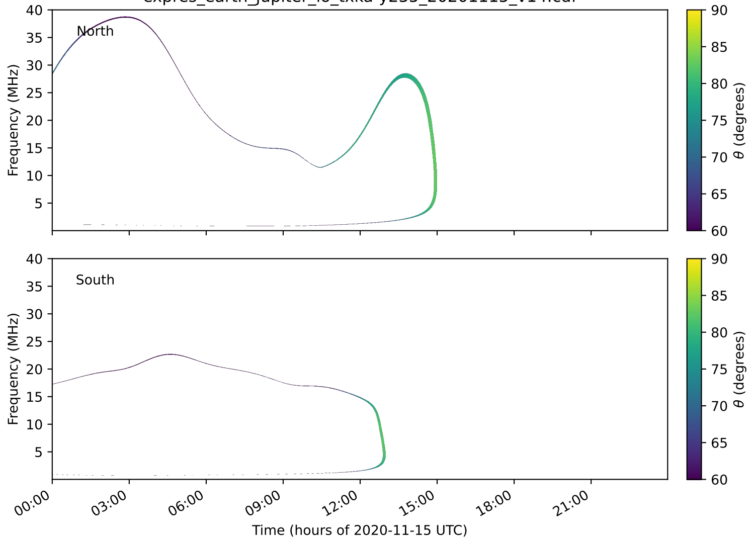
expres_earth_jupiter_io_txka-y235_20201115_v14.cdf
