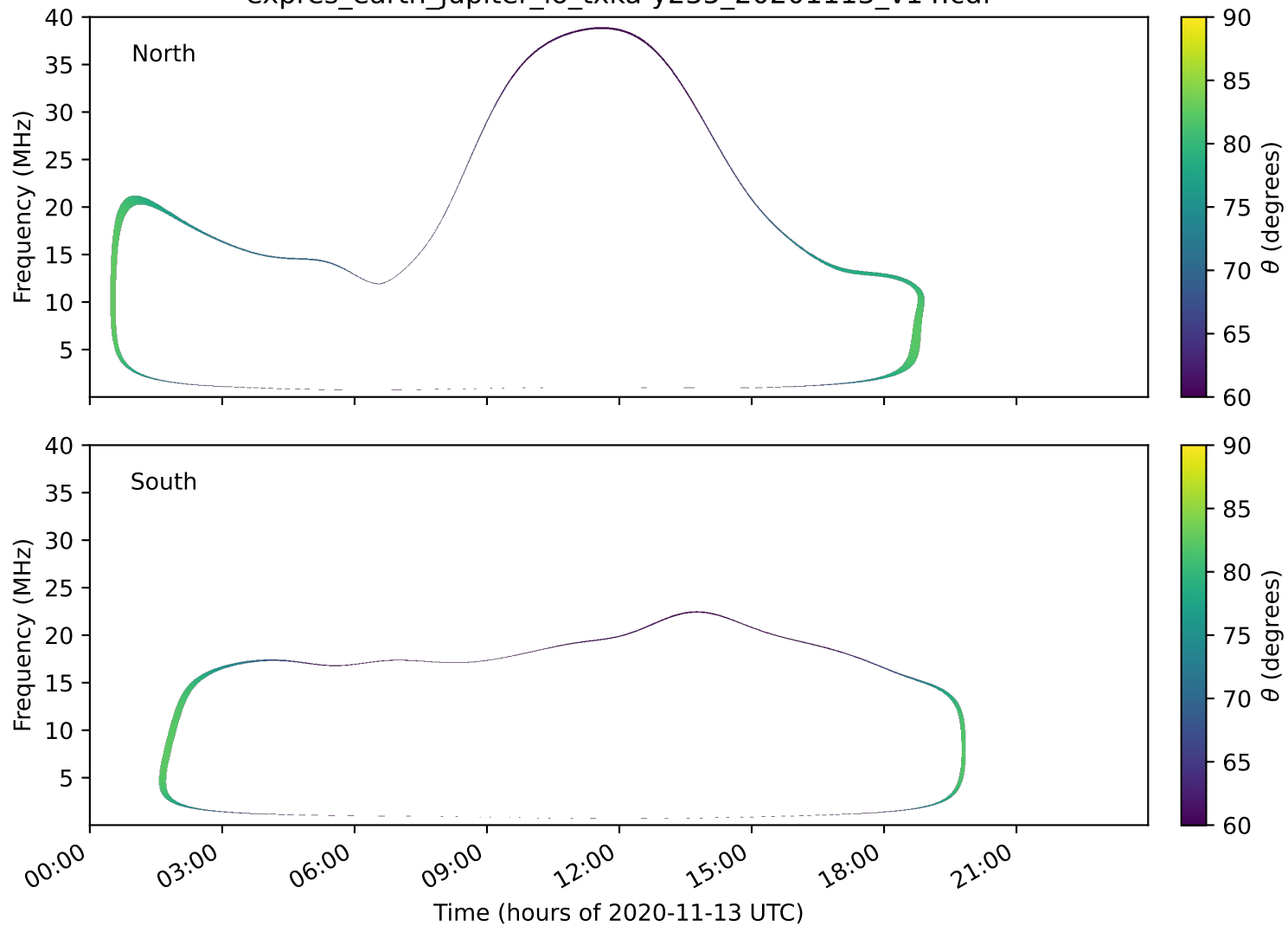
expres_earth_jupiter_io_txka-y235_20201113_v14.cdf
