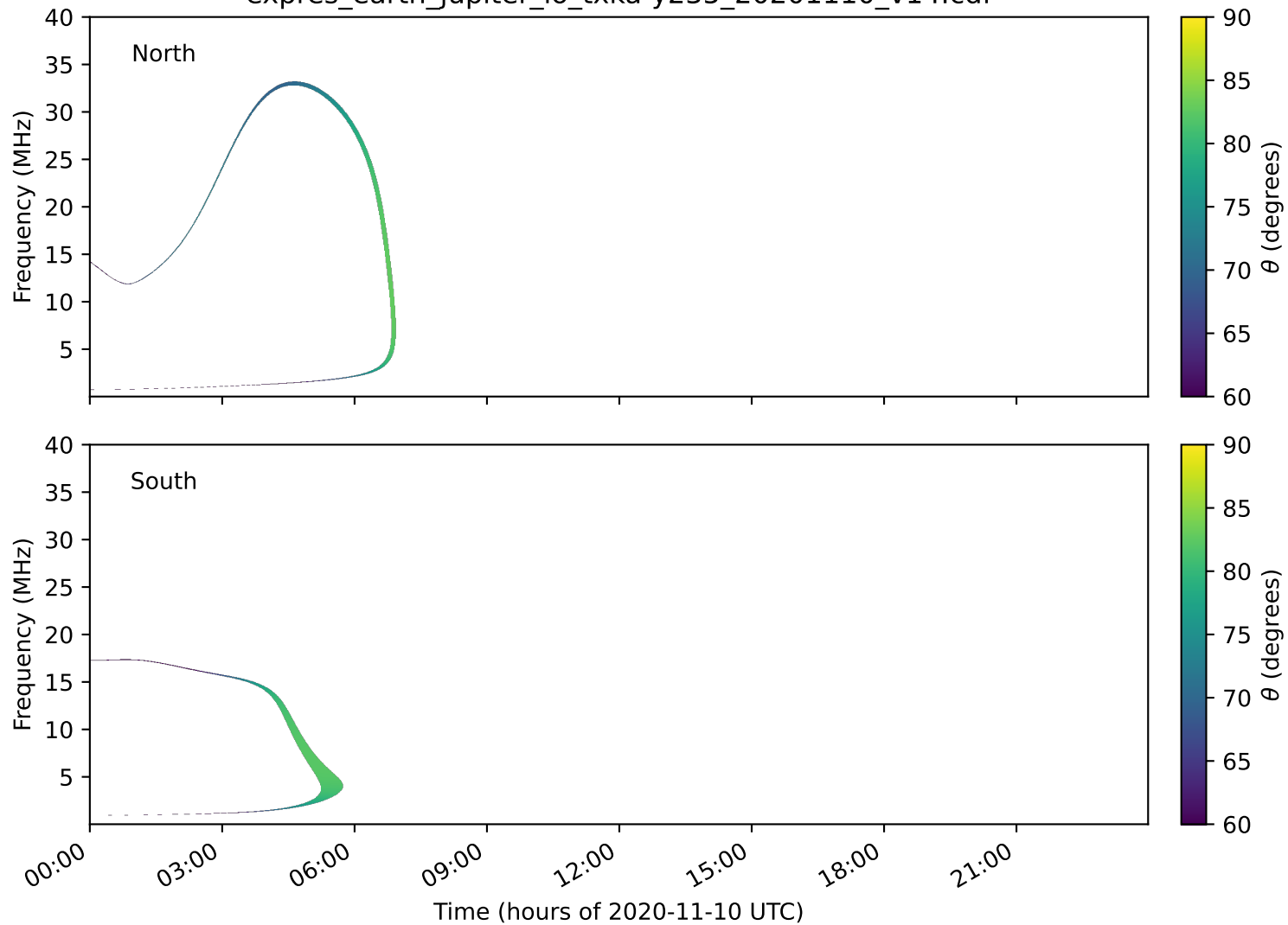
expres_earth_jupiter_io_txka-y235_20201110_v14.cdf
