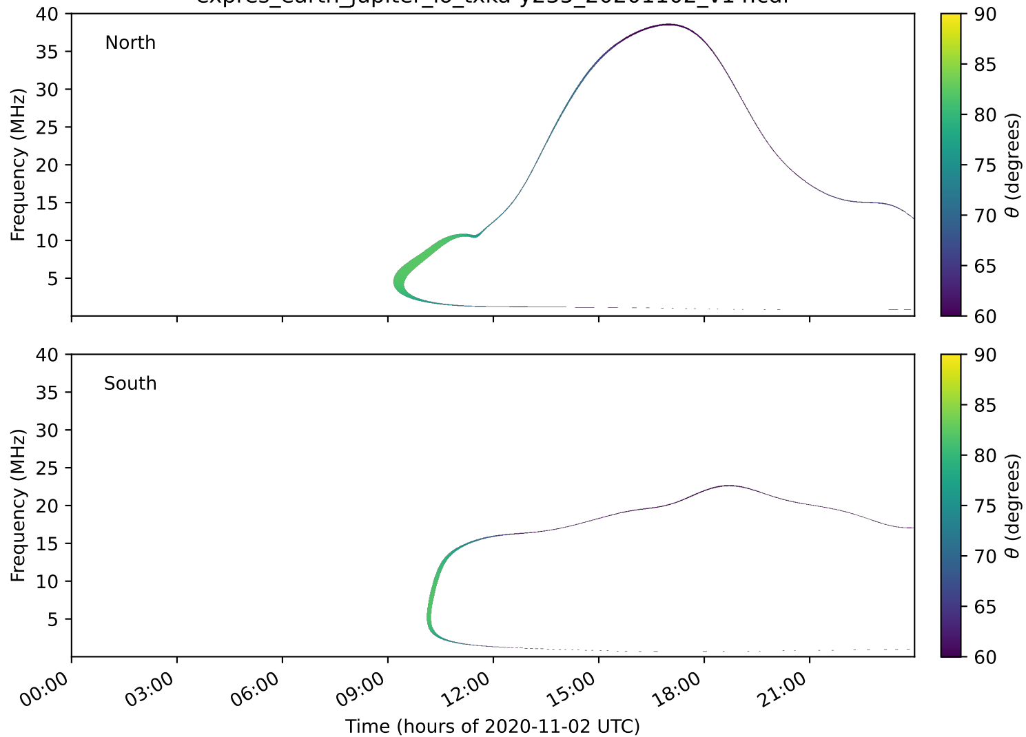
expres_earth_jupiter_io_txka-y235_20201102_v14.cdf
