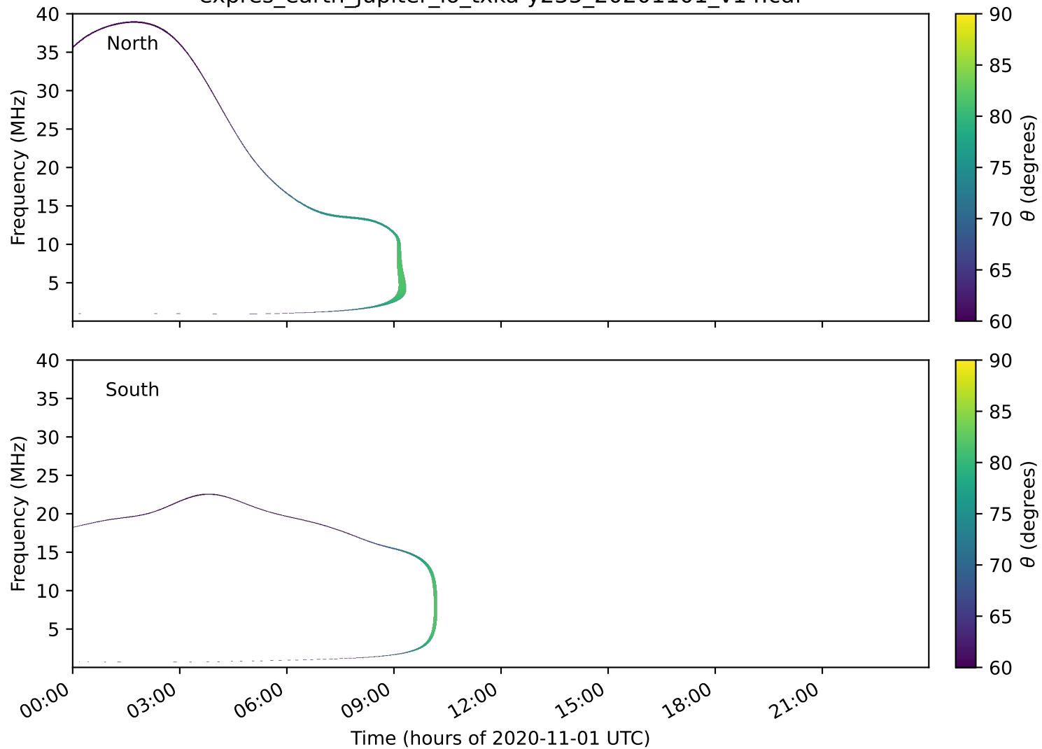
expres_earth_jupiter_io_txka-y235_20201101_v14.cdf
