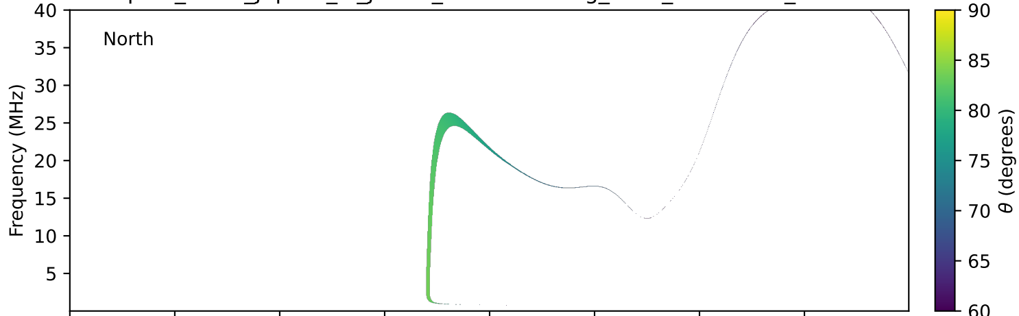
expres_earth_jupiter_io_jrm33_lossc-wid1deg_3kev_20201125_v11.cdf
