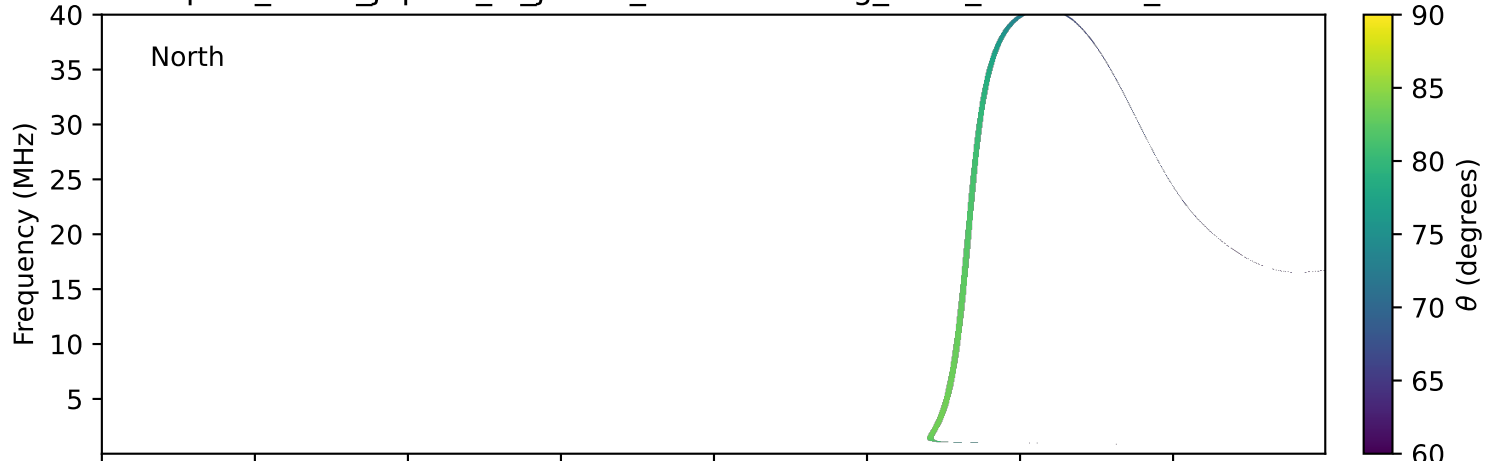
expres_earth_jupiter_io_jrm33_lossc-wid1deg_3kev_20201123_v11.cdf
