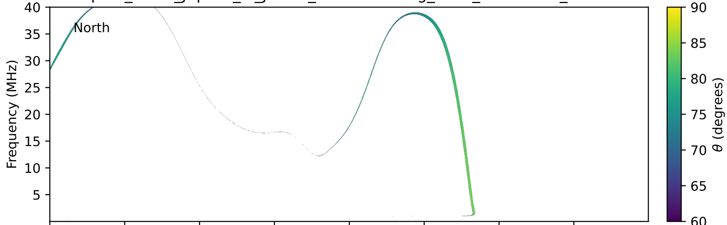
expres_earth_jupiter_io_jrm33_lossc-wid1deg_3kev_20201122_v11.cdf
