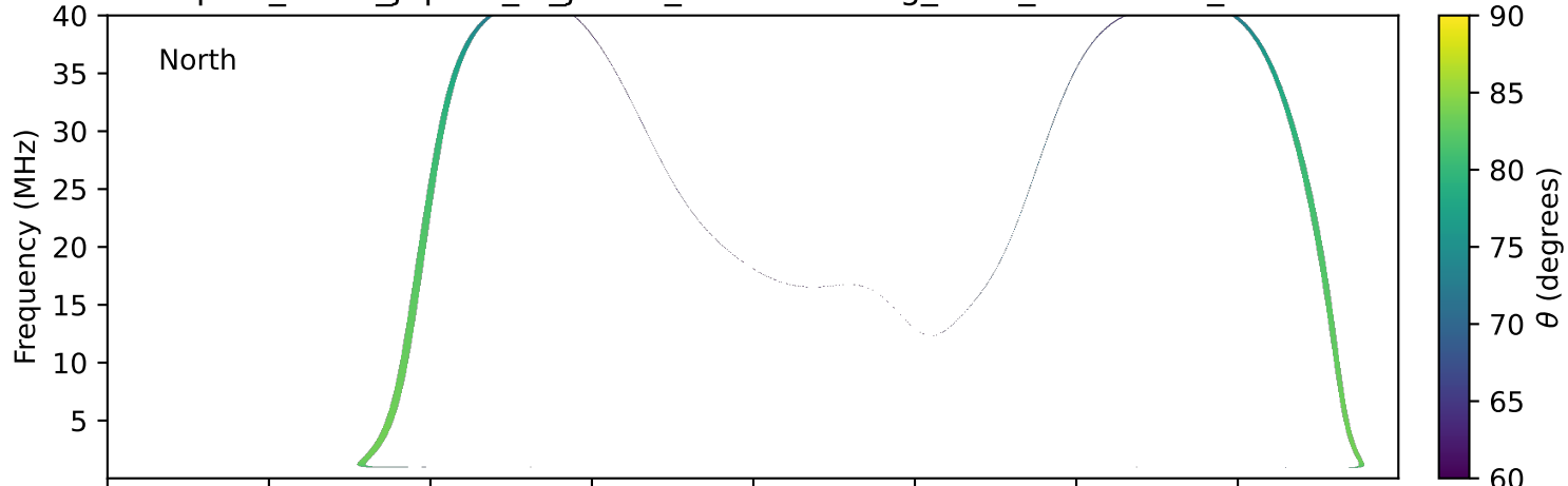
expres_earth_jupiter_io_jrm33_lossc-wid1deg_3kev_20201104_v11.cdf
