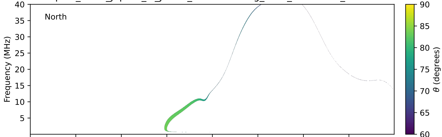
expres_earth_jupiter_io_jrm33_lossc-wid1deg_3kev_20201102_v11.cdf
