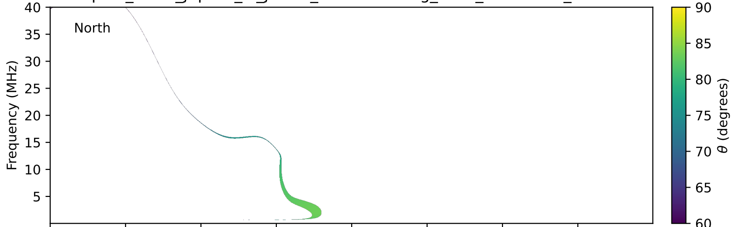
expres_earth_jupiter_io_jrm33_lossc-wid1deg_3kev_20201101_v11.cdf
