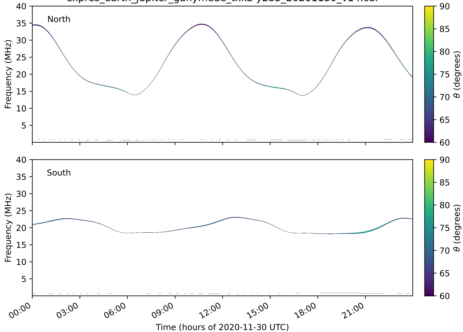
expres_earth_jupiter_ganymede_txka-y235_20201130_v14.cdf
