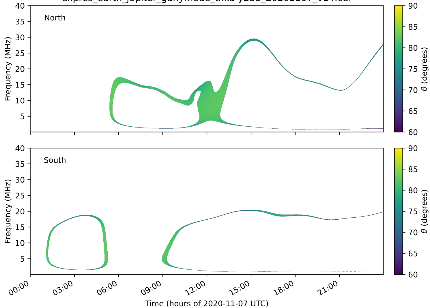
expres_earth_jupiter_ganymede_txka-y235_20201107_v14.cdf
