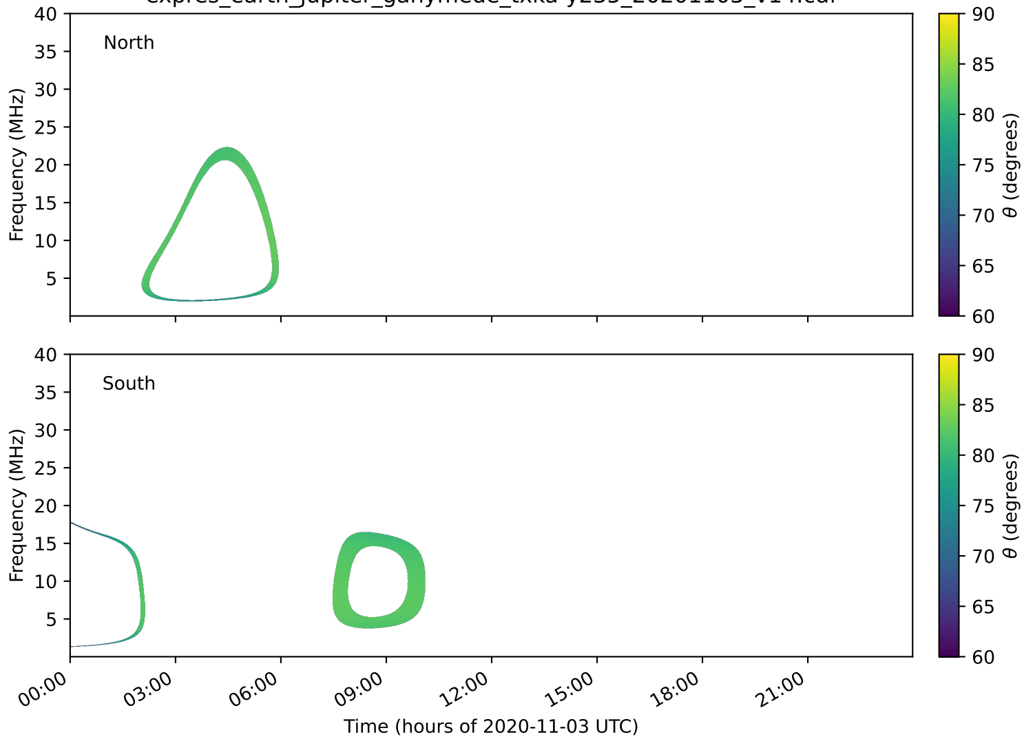
expres_earth_jupiter_ganymede_txka-y235_20201103_v14.cdf
