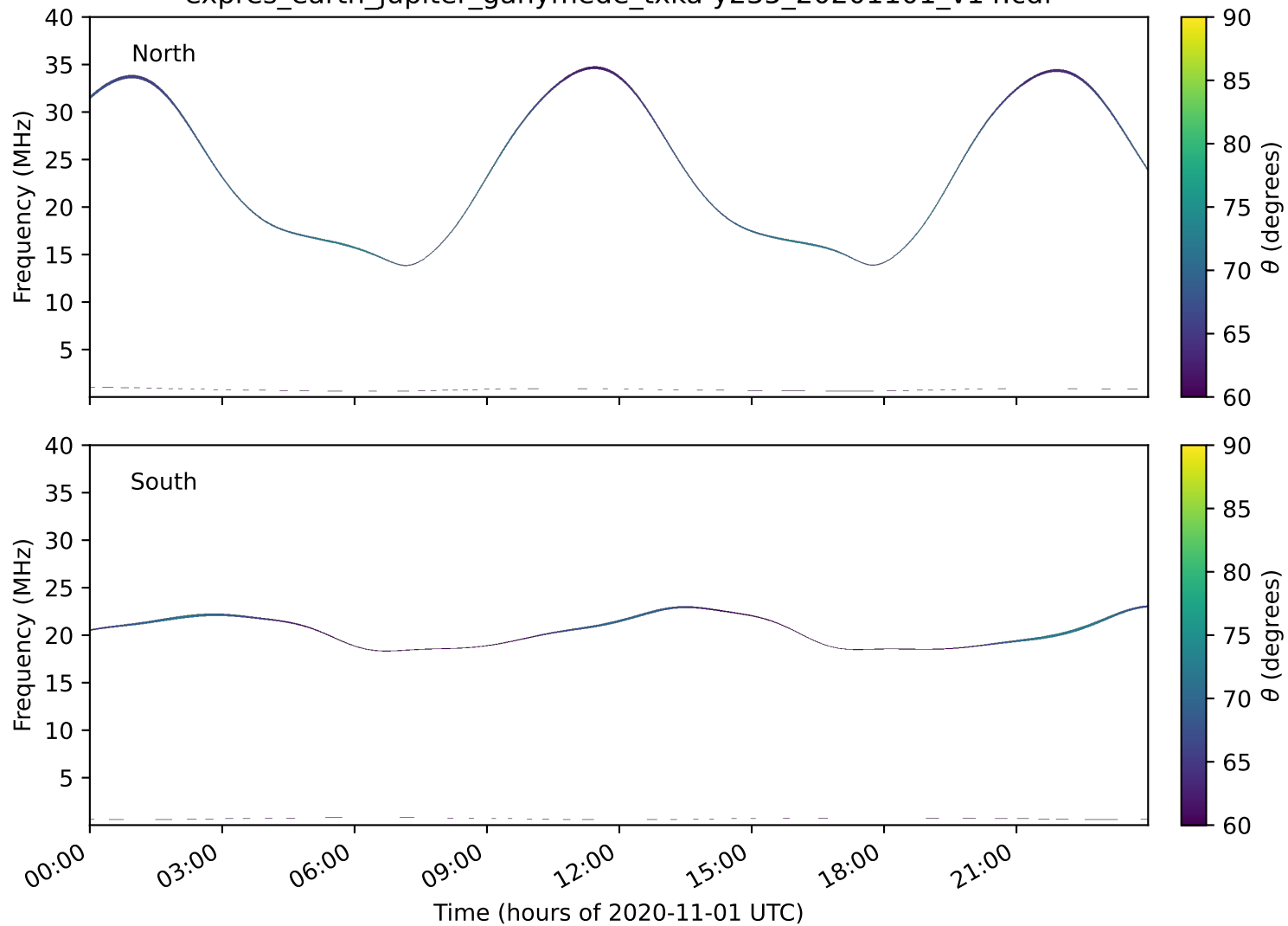
expres_earth_jupiter_ganymede_txka-y235_20201101_v14.cdf
