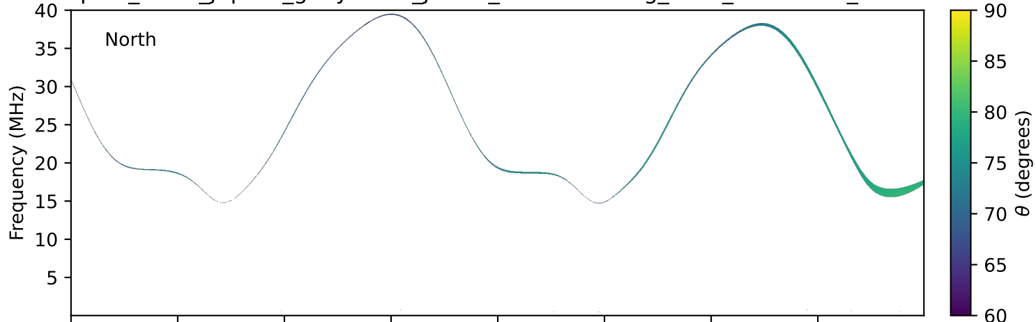
expres_earth_jupiter_ganymede_jrm33_lossc-wid1deg_3kev_20201109_v11.cdf
