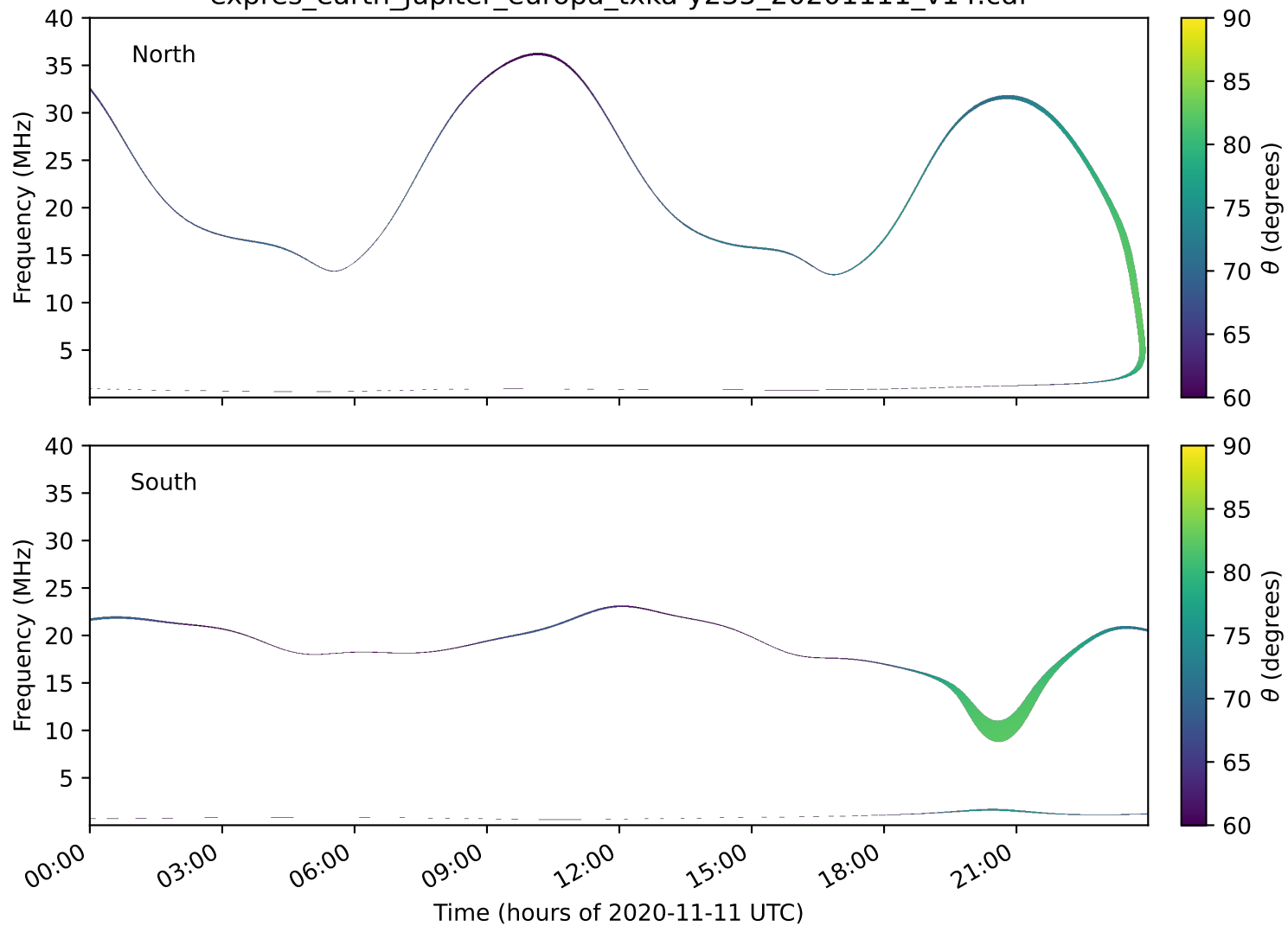
expres_earth_jupiter_europa_txka-y235_20201111_v14.cdf
