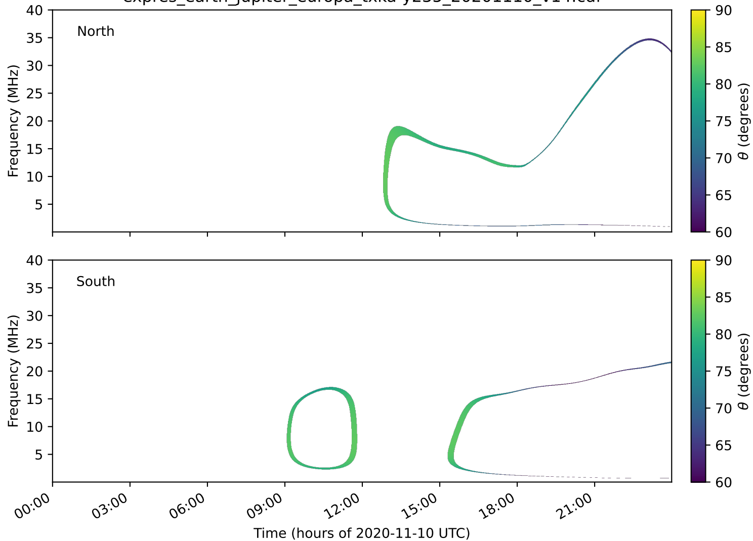
expres_earth_jupiter_europa_txka-y235_20201110_v14.cdf
