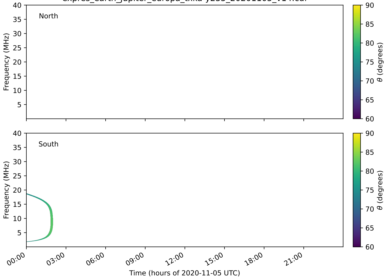
expres_earth_jupiter_europa_txka-y235_20201105_v14.cdf
