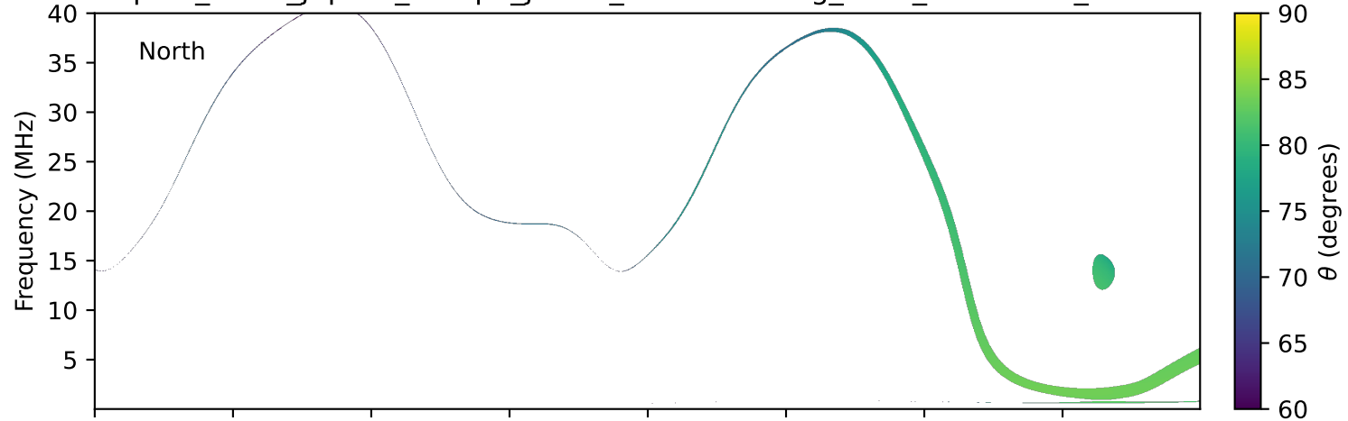
expres_earth_jupiter_europa_jrm33_lossc-wid1deg_3kev_20201129_v11.cdf
