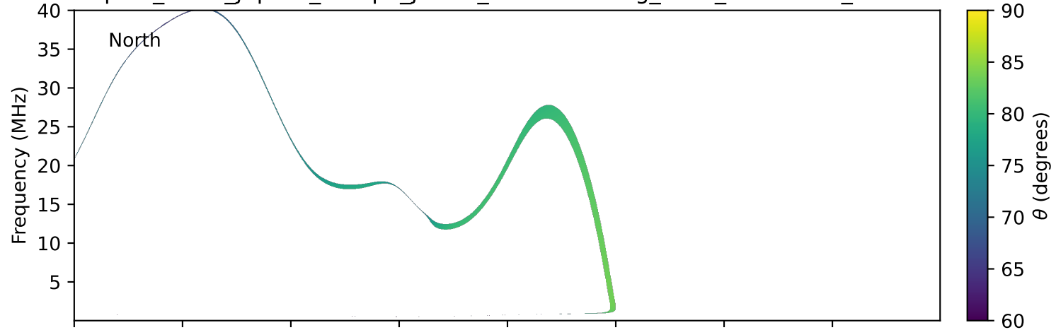
expres_earth_jupiter_europa_jrm33_lossc-wid1deg_3kev_20201108_v11.cdf
