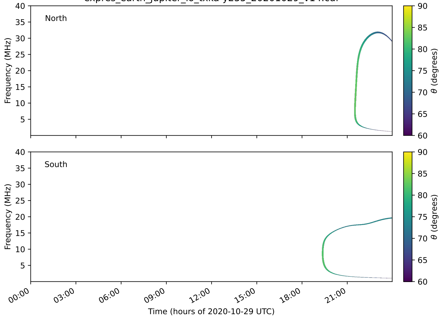
expres_earth_jupiter_io_txka-y235_20201029_v14.cdf
