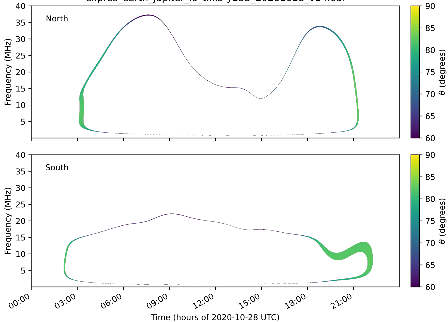
expres_earth_jupiter_io_txka-y235_20201028_v14.cdf
