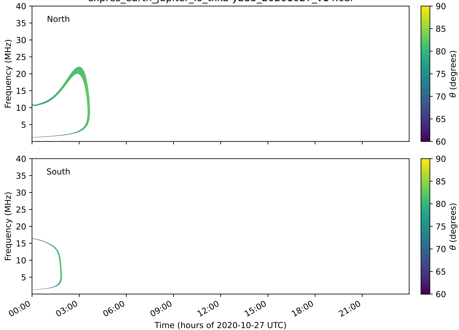
expres_earth_jupiter_io_txka-y235_20201027_v14.cdf
