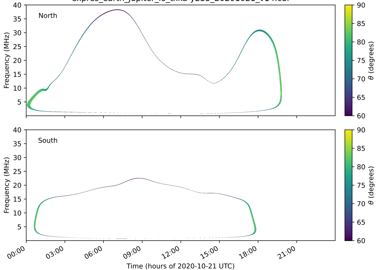
expres_earth_jupiter_io_txka-y235_20201021_v14.cdf
