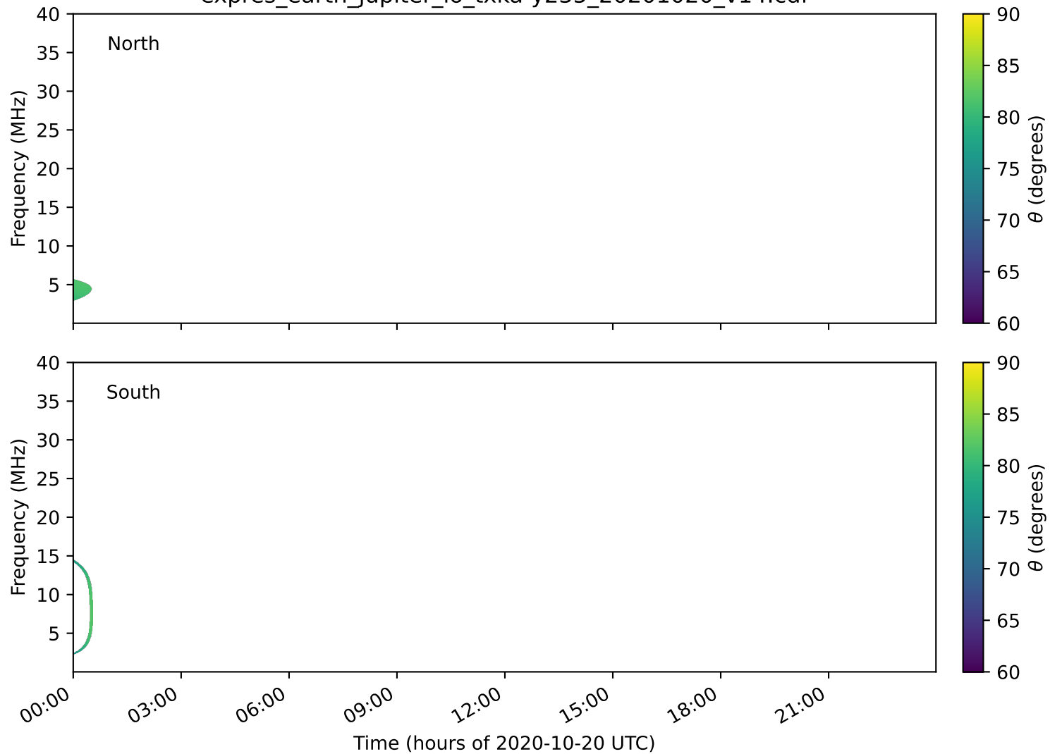
expres_earth_jupiter_io_txka-y235_20201020_v14.cdf
