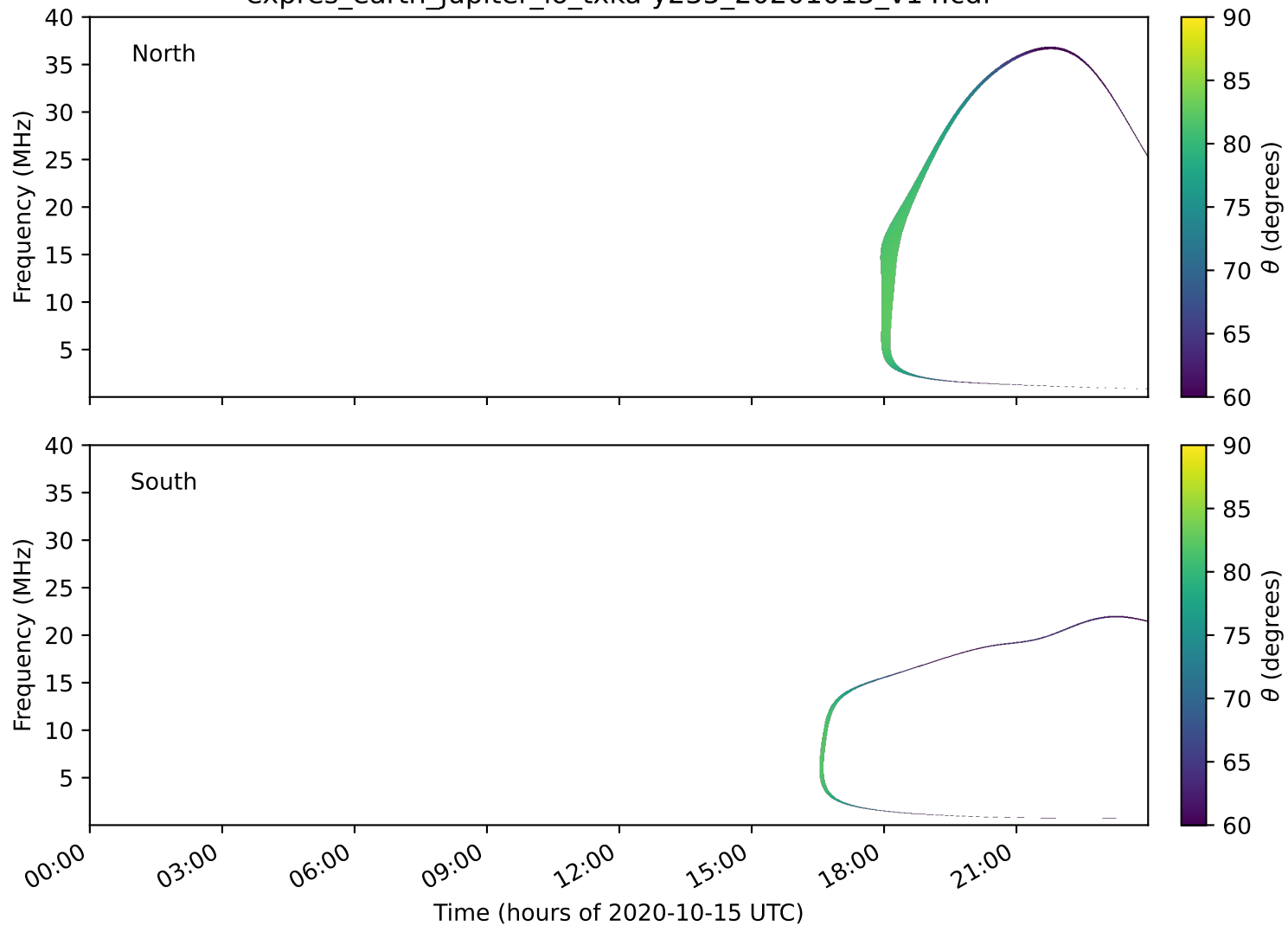
expres_earth_jupiter_io_txka-y235_20201015_v14.cdf
