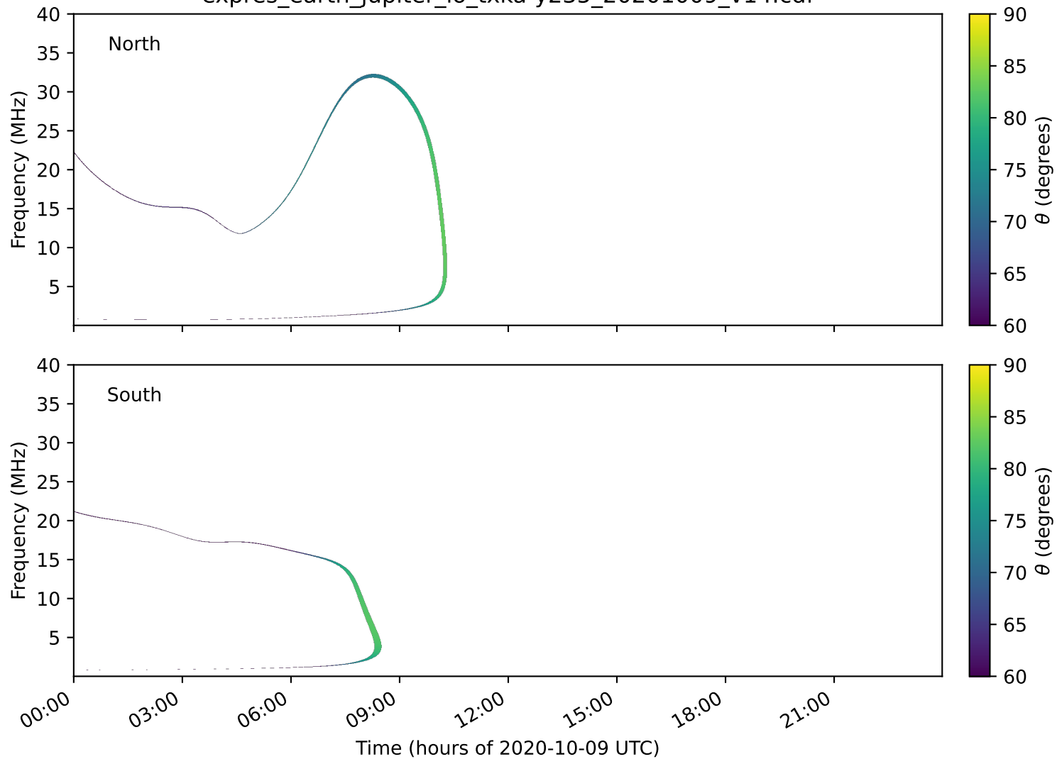
expres_earth_jupiter_io_txka-y235_20201009_v14.cdf
