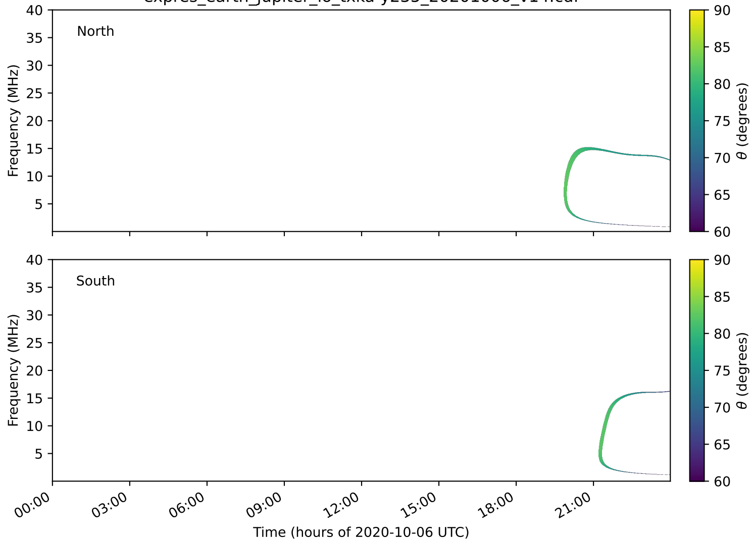
expres_earth_jupiter_io_txka-y235_20201006_v14.cdf
