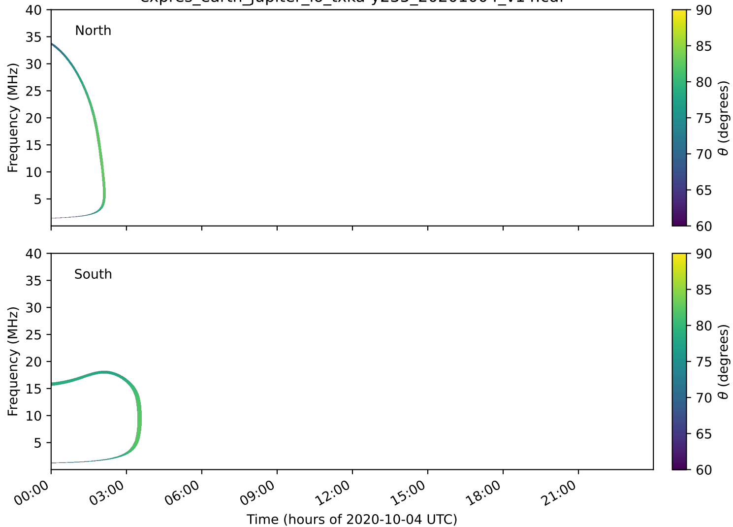
expres_earth_jupiter_io_txka-y235_20201004_v14.cdf
