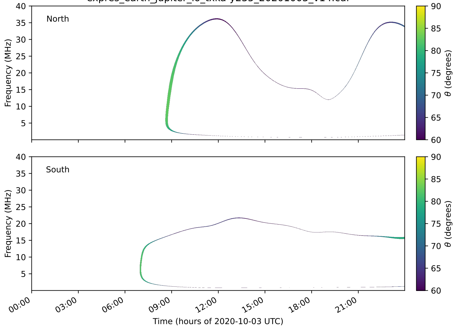
expres_earth_jupiter_io_txka-y235_20201003_v14.cdf
