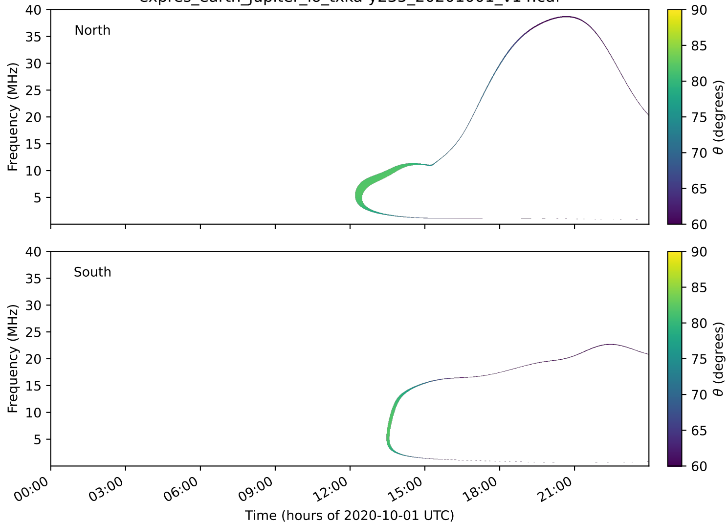
expres_earth_jupiter_io_txka-y235_20201001_v14.cdf
