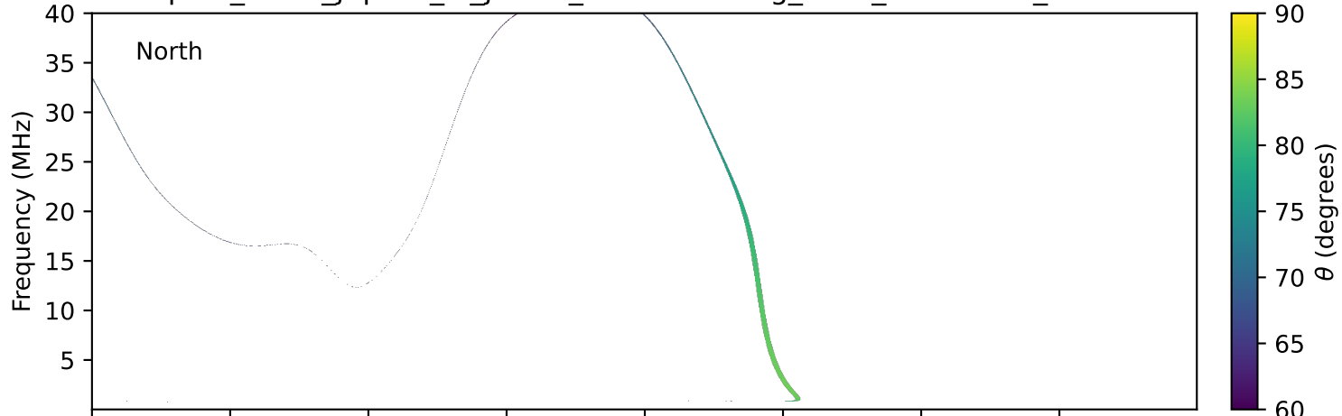
expres_earth_jupiter_io_jrm33_lossc-wid1deg_3kev_20201030_v11.cdf
