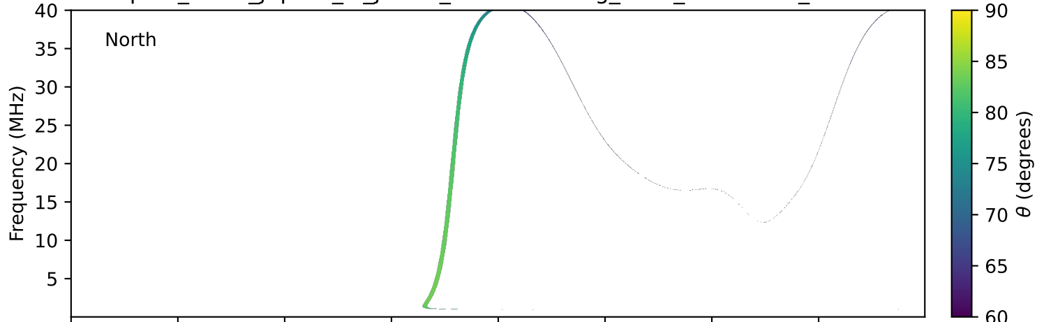
expres_earth_jupiter_io_jrm33_lossc-wid1deg_3kev_20201010_v11.cdf
