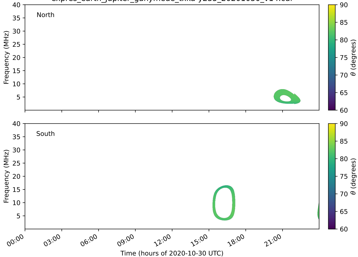
expres_earth_jupiter_ganymede_txka-y235_20201030_v14.cdf
