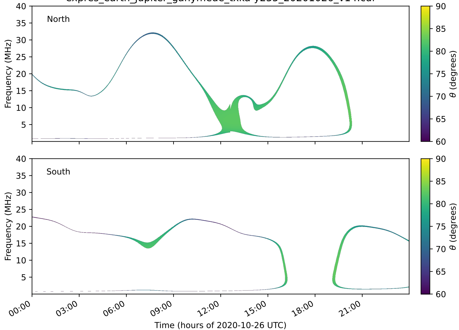
expres_earth_jupiter_ganymede_txka-y235_20201026_v14.cdf
