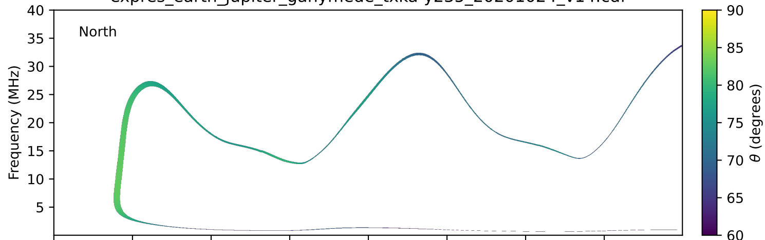
expres_earth_jupiter_ganymede_txka-y235_20201024_v14.cdf
