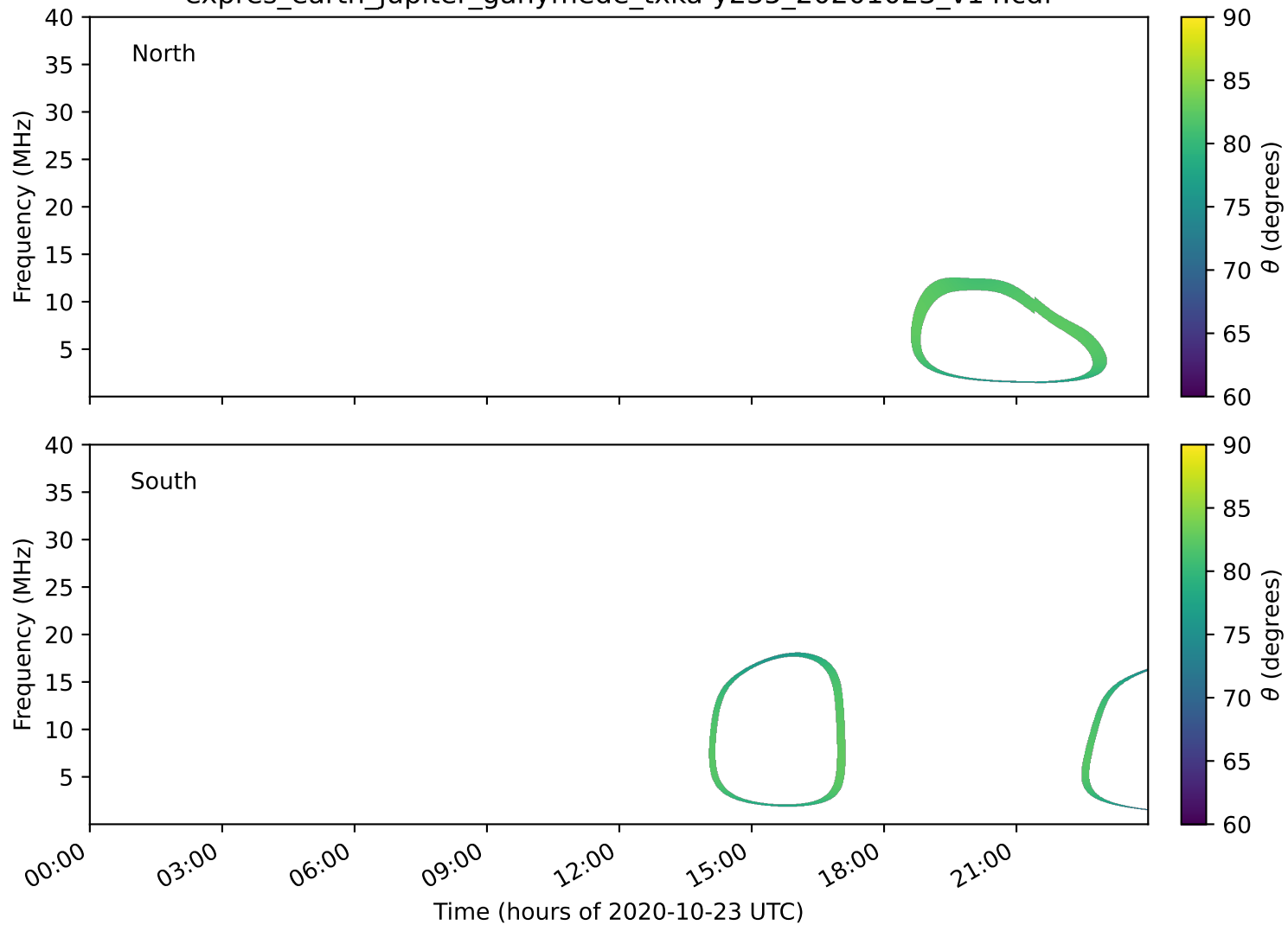
expres_earth_jupiter_ganymede_txka-y235_20201023_v14.cdf
