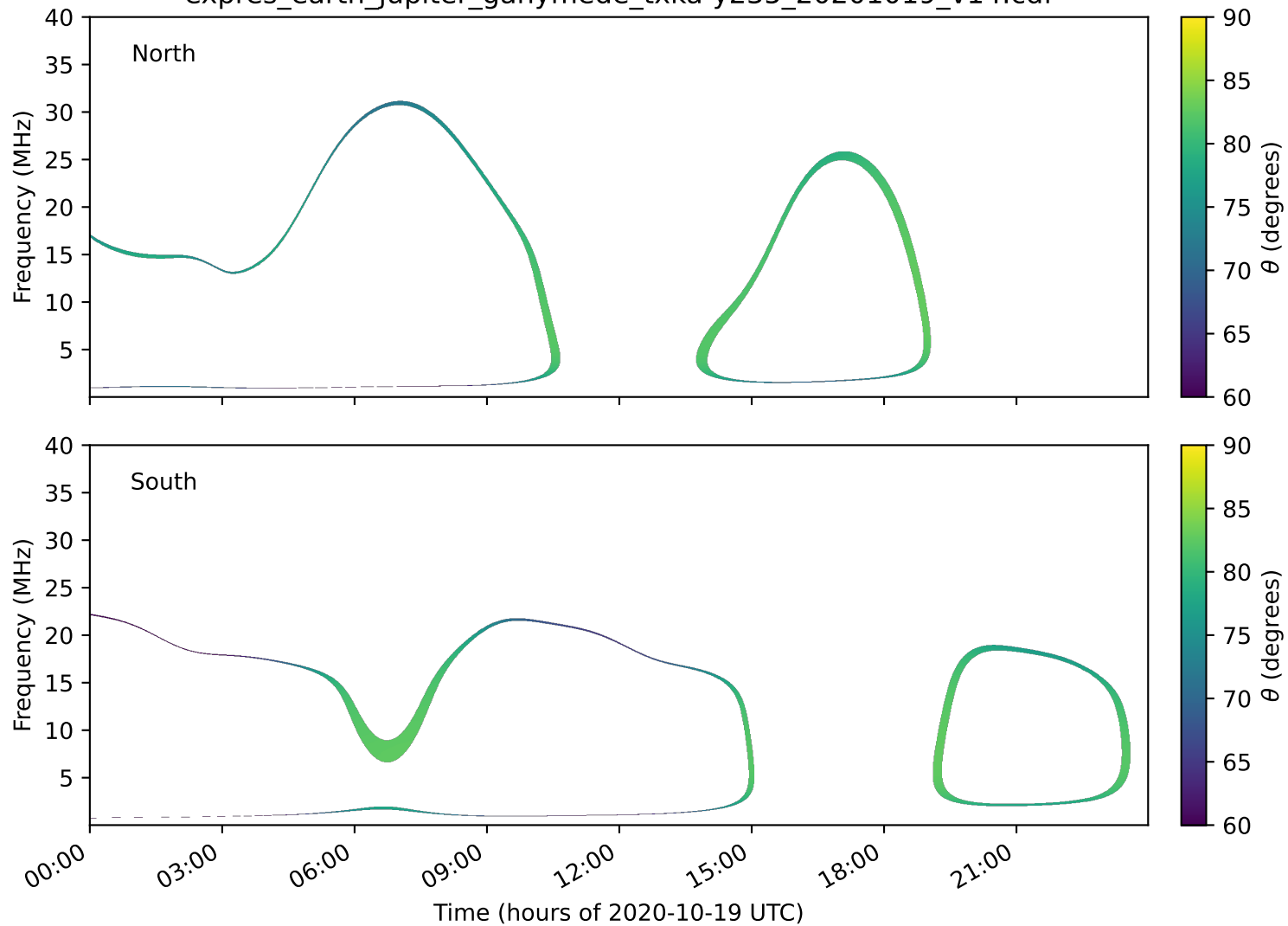
expres_earth_jupiter_ganymede_txka-y235_20201019_v14.cdf
