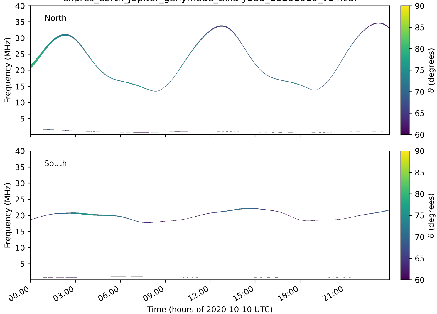
expres_earth_jupiter_ganymede_txka-y235_20201010_v14.cdf
