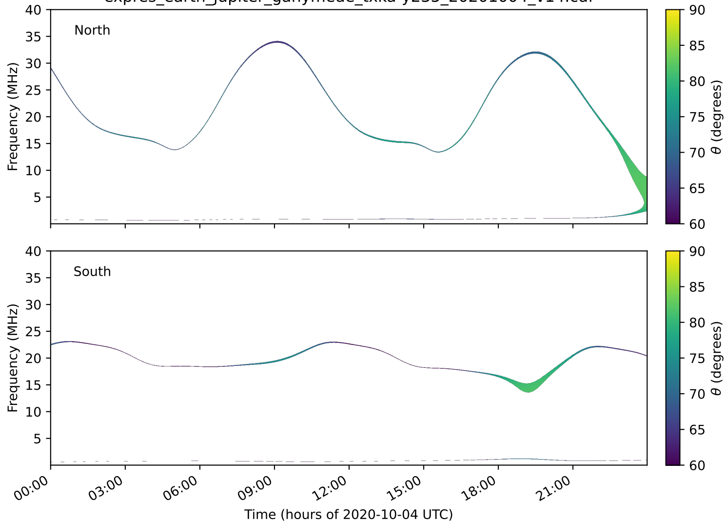
expres_earth_jupiter_ganymede_txka-y235_20201004_v14.cdf
