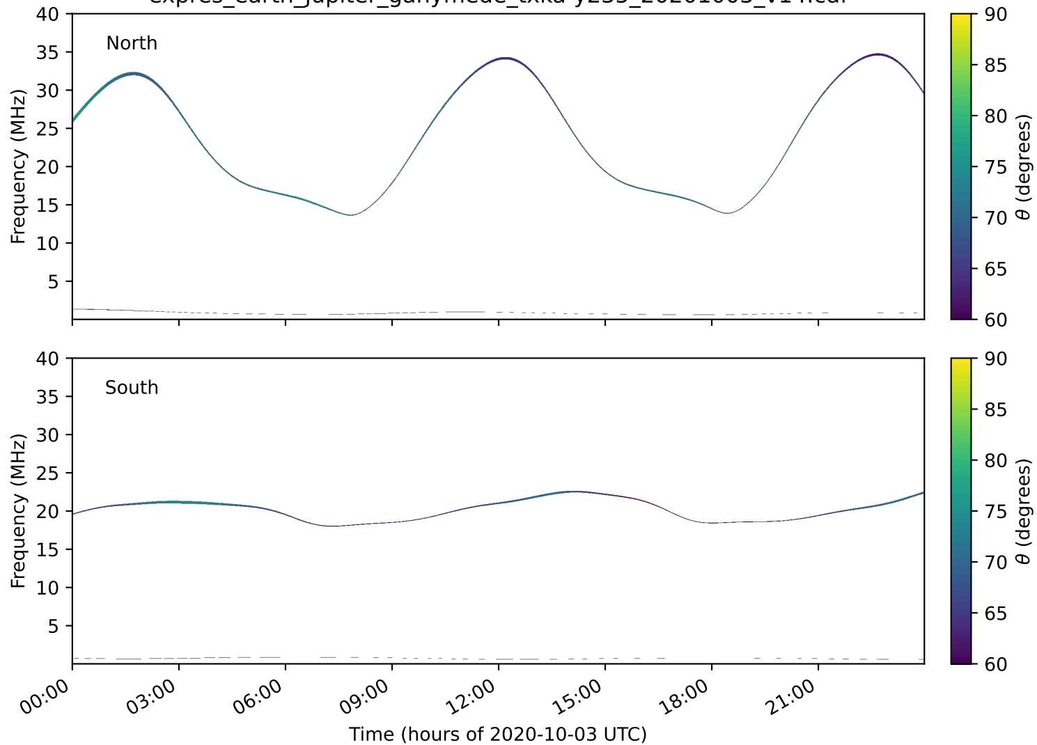
expres_earth_jupiter_ganymede_txka-y235_20201003_v14.cdf
