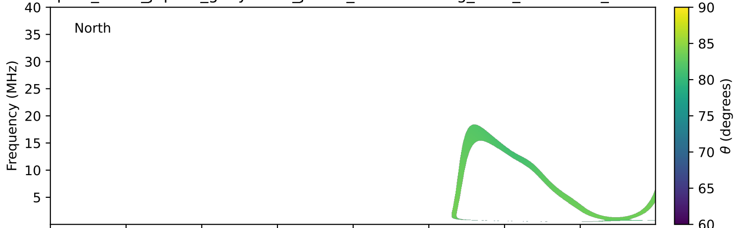
expres_earth_jupiter_ganymede_jrm33_lossc-wid1deg_3kev_20201009_v11.cdf
