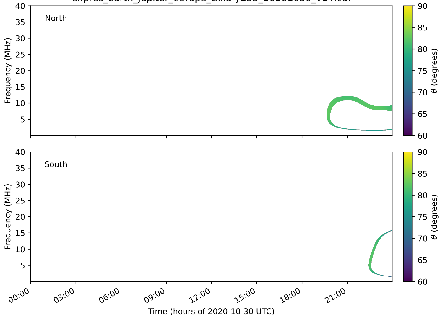
expres_earth_jupiter_europa_txka-y235_20201030_v14.cdf
