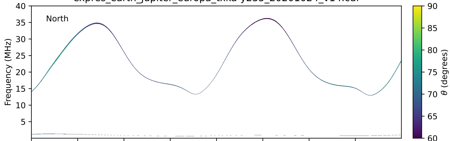
expres_earth_jupiter_europa_txka-y235_20201024_v14.cdf
