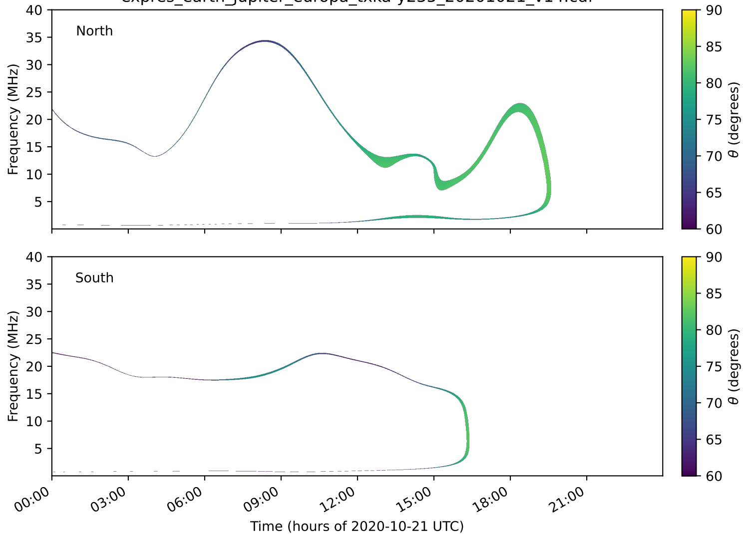
expres_earth_jupiter_europa_txka-y235_20201021_v14.cdf
