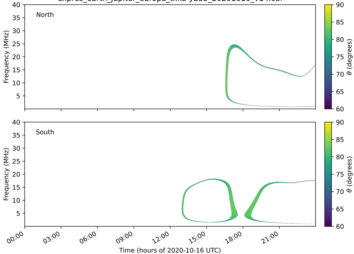
expres_earth_jupiter_europa_txka-y235_20201016_v14.cdf
