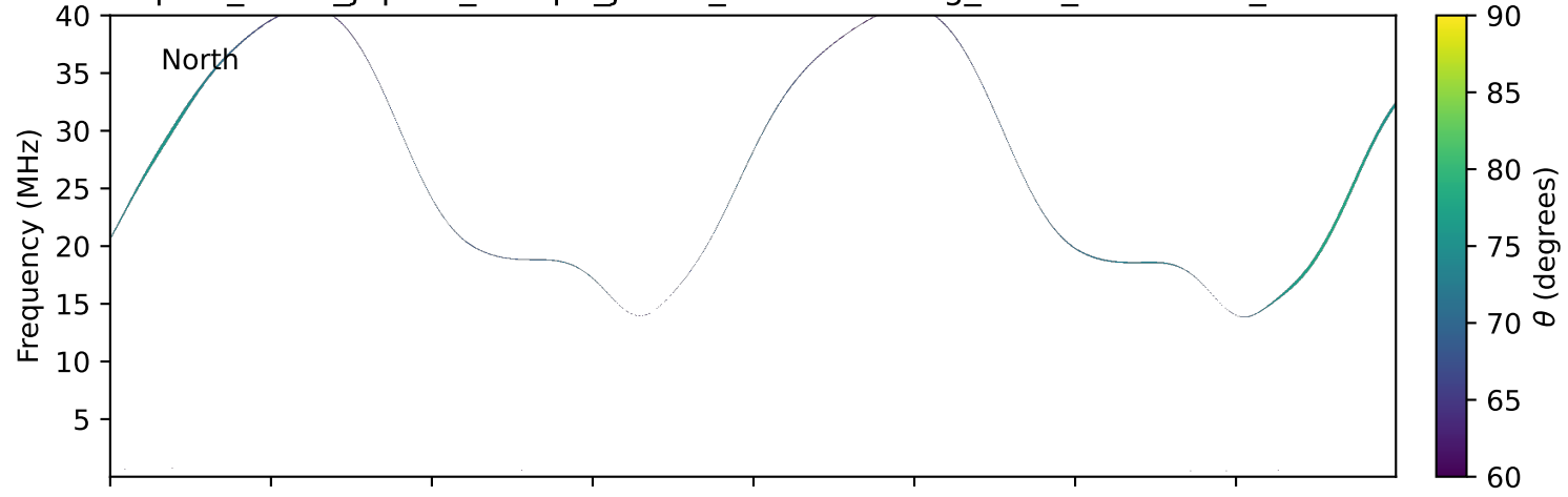
expres_earth_jupiter_europa_jrm33_lossc-wid1deg_3kev_20201017_v11.cdf
